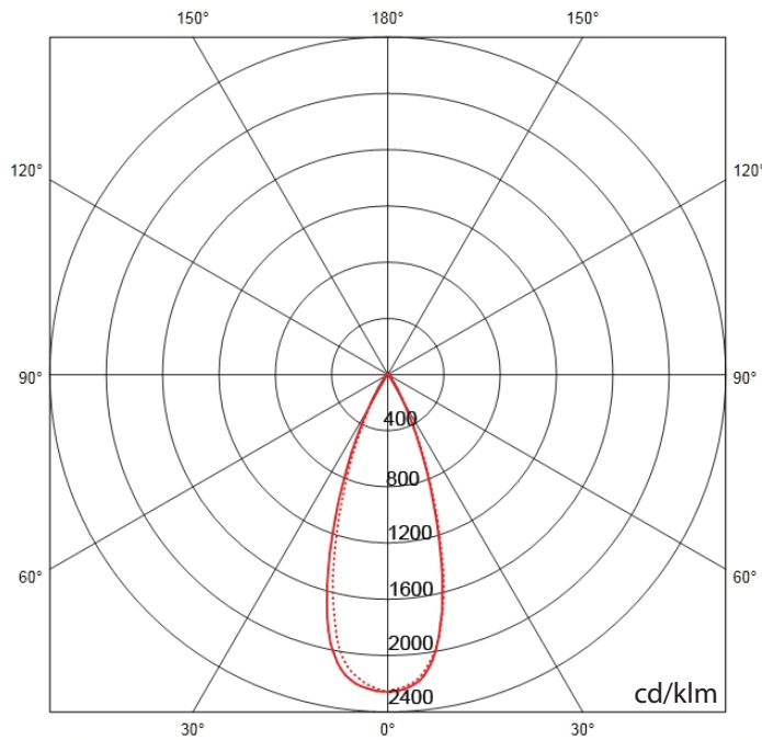
Metrolight With Lens (45°)
