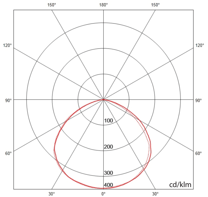
Metrolight Without Lens (120°)
